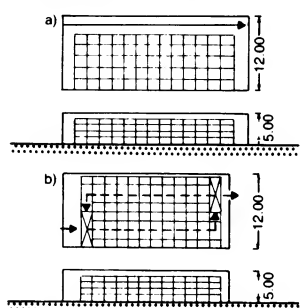
⑧ a) Block store with optimal space/height usage b) Block store in rotation
